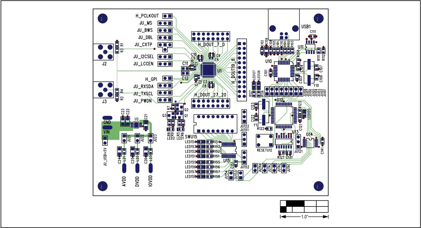
Figure 12. MAX9272 Coax EV Kit PCB Layout—Component Side
