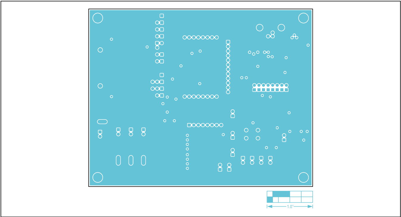
Figure 13. MAX9272 Coax EV Kit PCB Layout—Ground Layer 2
