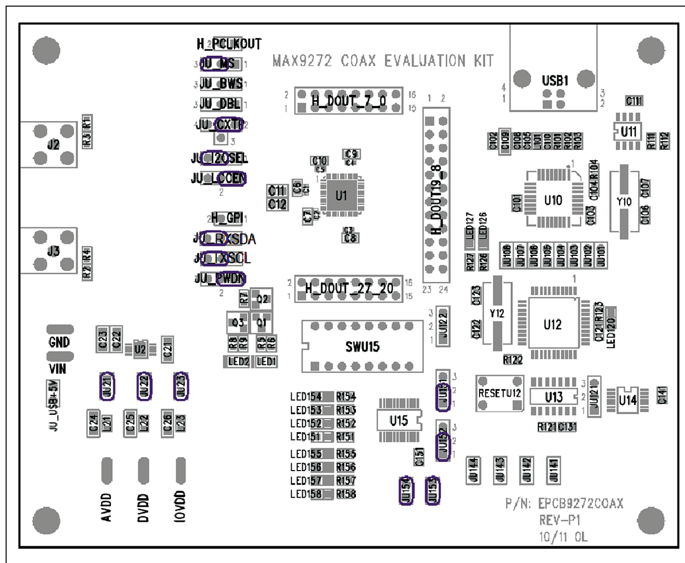
Figure 9. Initial Jumper Settings for I 2 C Mode
