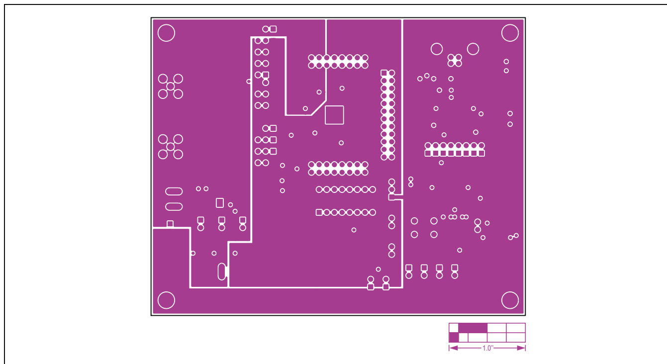
Figure 14. MAX9272 Coax EV Kit PCB Layout—Power Layer 3
