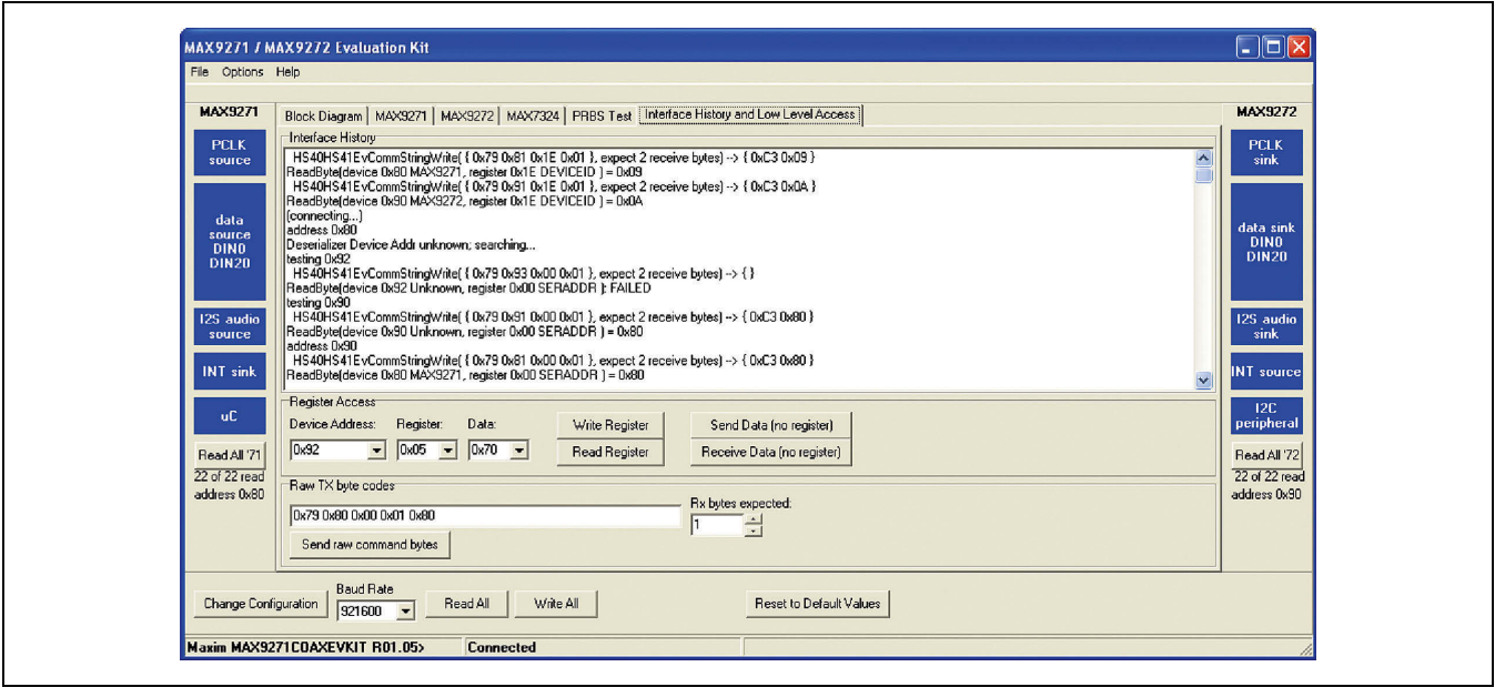
Figure 6. MAX9271 EV Kit Software Main Window (Interface History and Low Level Access Tab)
