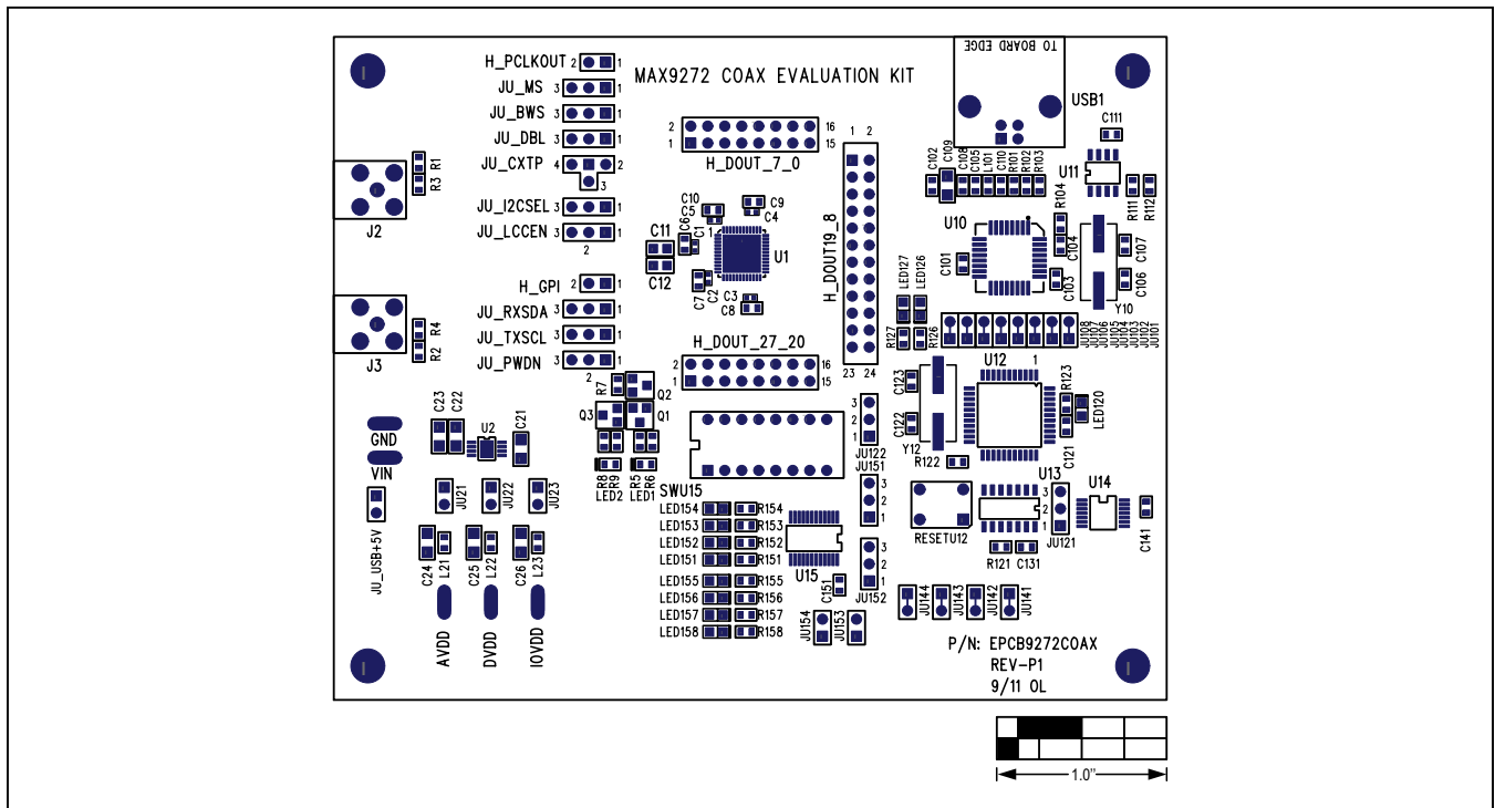
Figure 11. MAX9272 Coax EV Kit Component Placement Guide—Component Side
