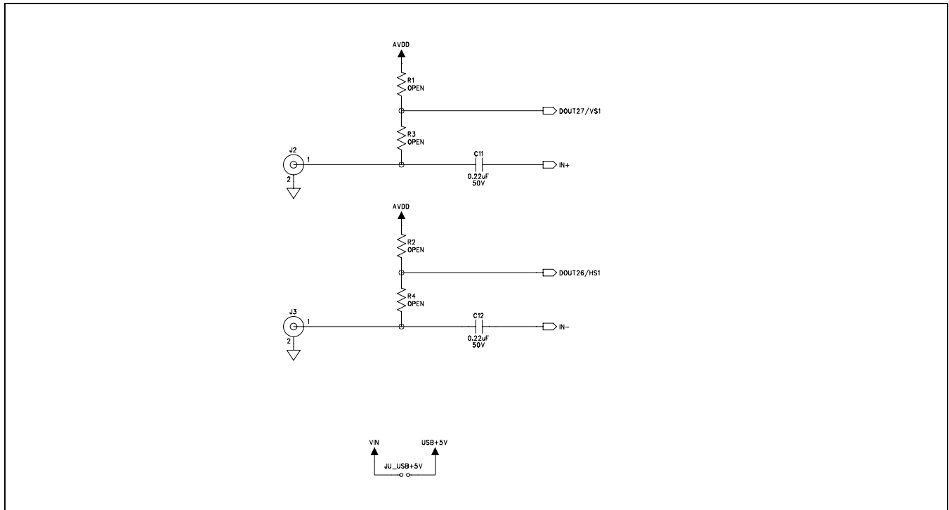
Figure 10c. MAX9272 Coax EV Kit Schematic (Sheet 3 of 3)
