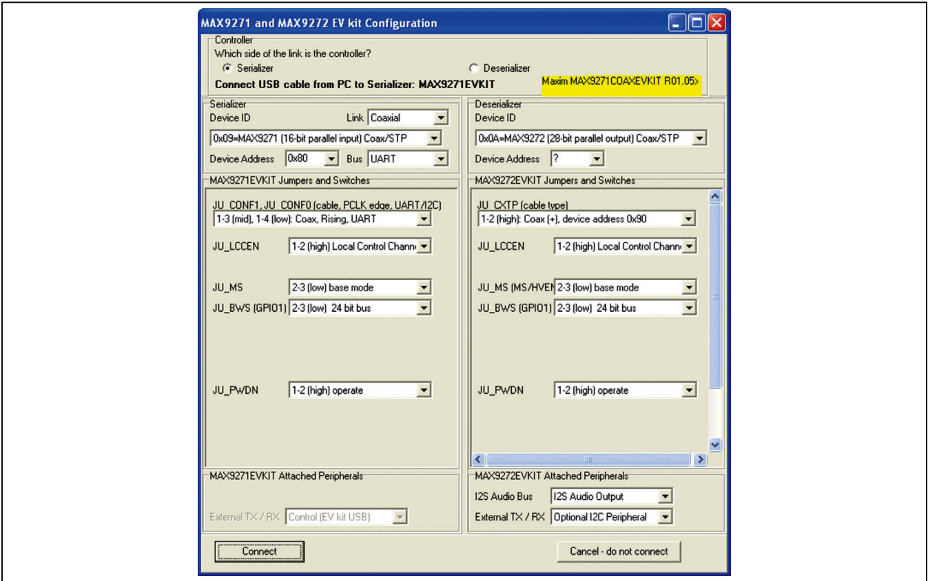
Figure 7. MAX9271/MAX9272 EV Kit Software Connect Window
