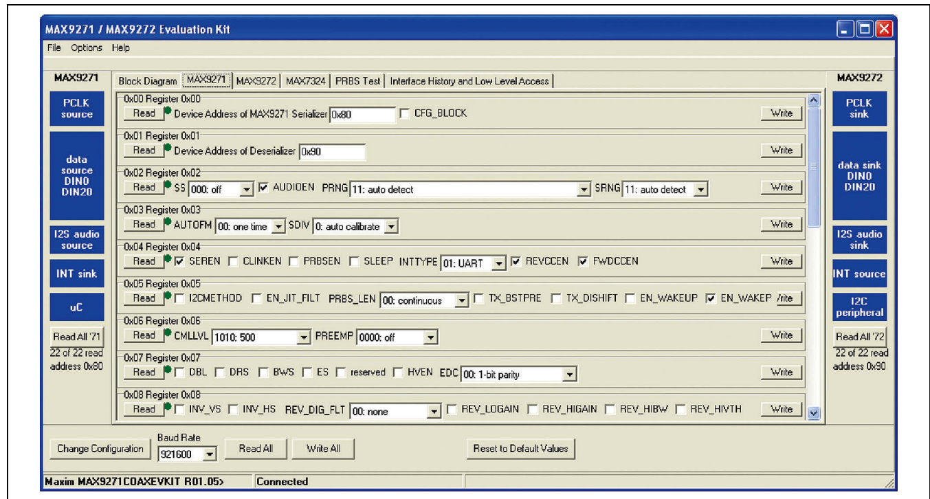
Figure 2. MAX9271/MAX9272 EV Kit Software Main Window (MAX9271 Tab)
