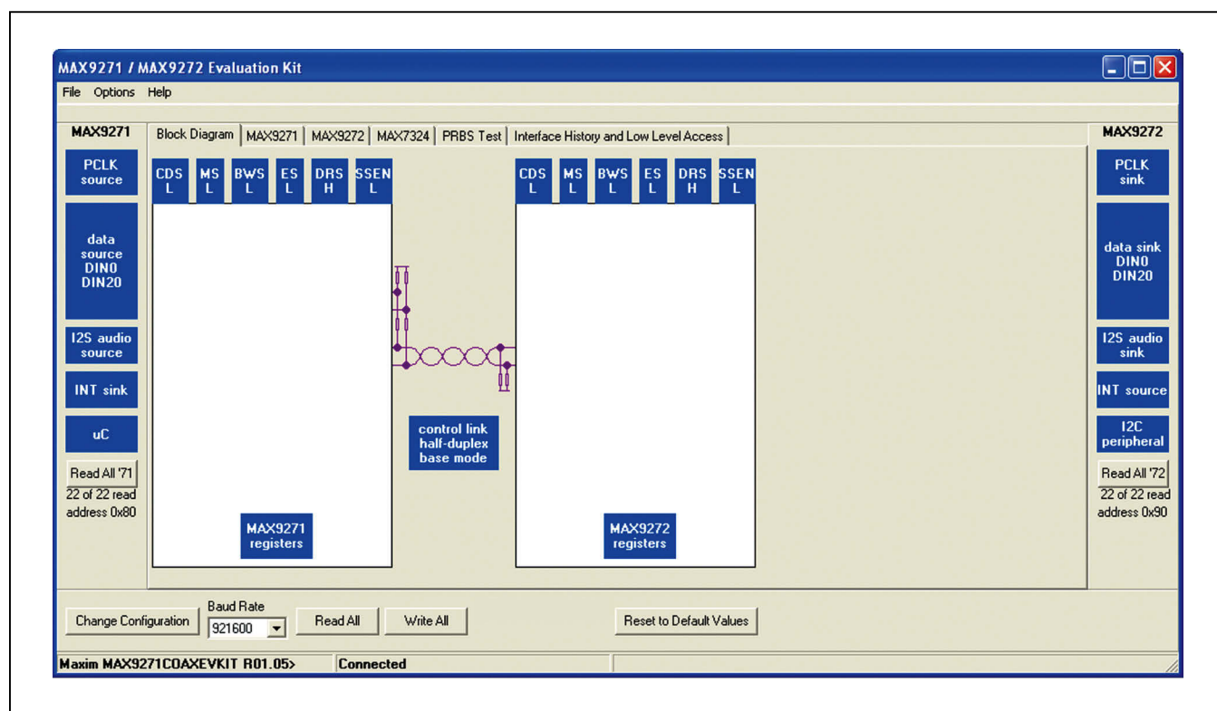
Figure 1. MAX9271/MAX9272 EV Kit Software Main Window (Block Diagram Tab)
