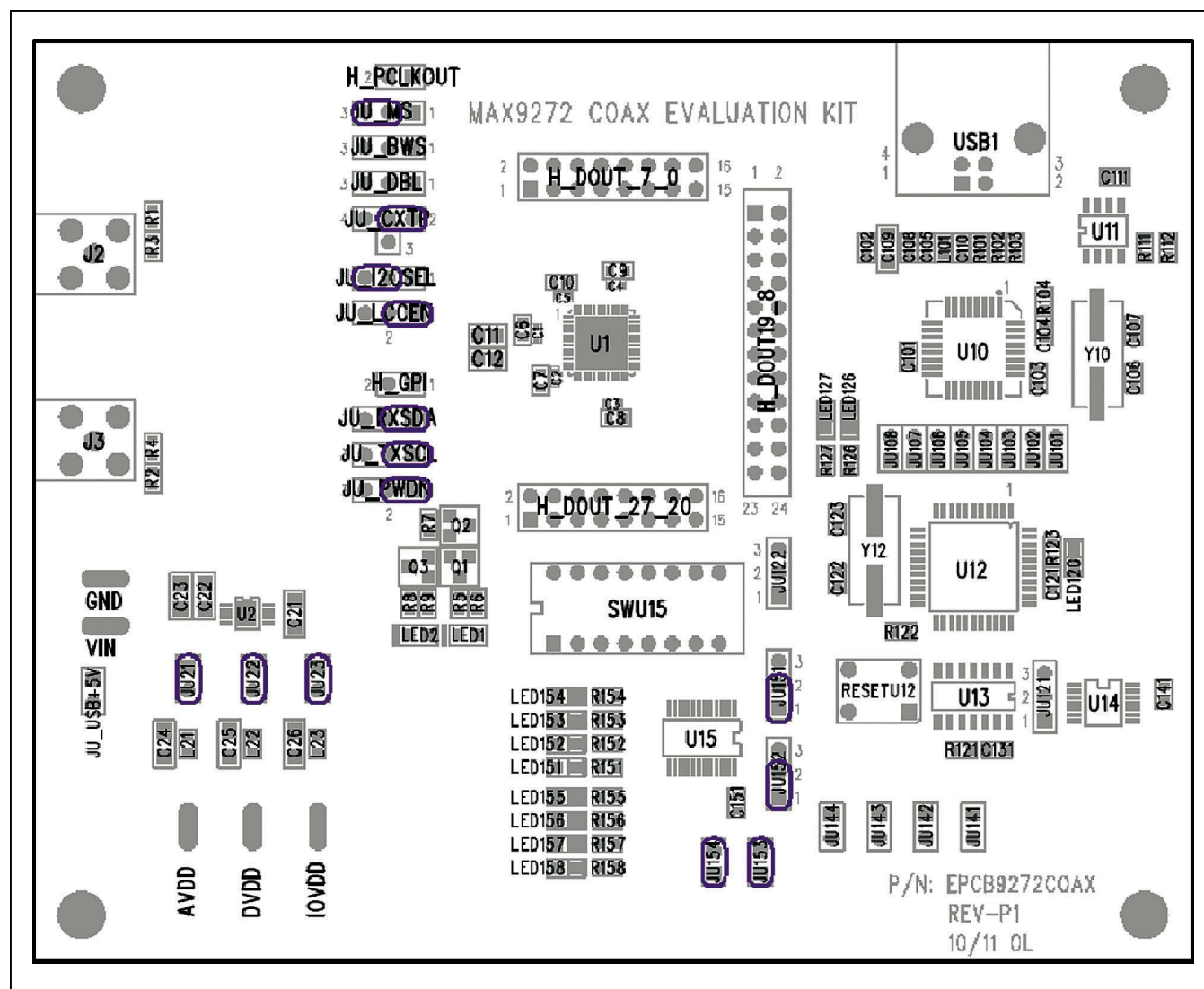
Figure 8. Initial Jumper Settings for UART Mode
