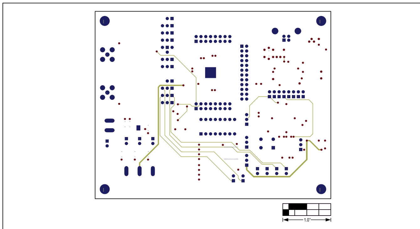
Figure 15. MAX9272 Coax EV Kit PCB Layout—Solder Side
